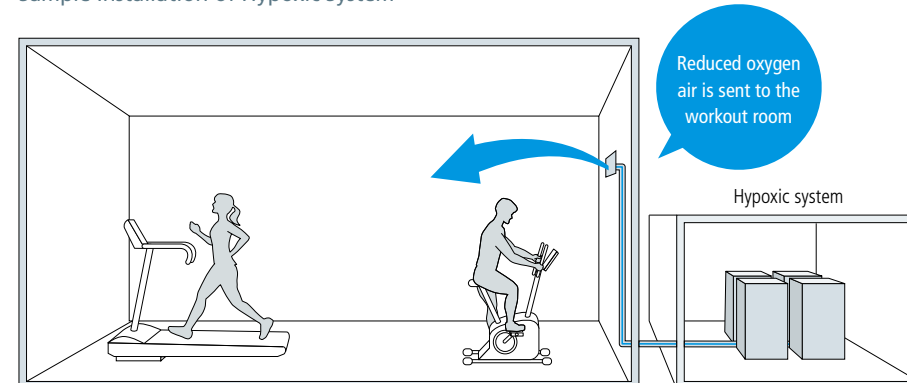
Sample Installation of Hypoxic System
